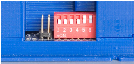
Abb. 25: OC32/NG DIPswitches
